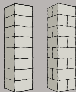
Massive pier 40 x 40 x 160 cm Tumbled / Brushed / Honed Massive pier with blind fuga 40 x 40 x 160 cm Tumbled / Brushed / Honed
